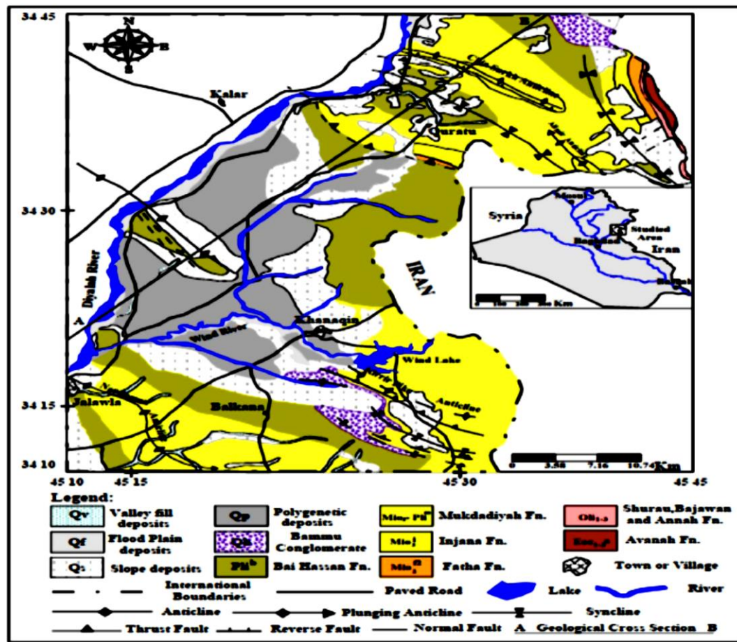
Figure (2): Geological map of studied area [10]
